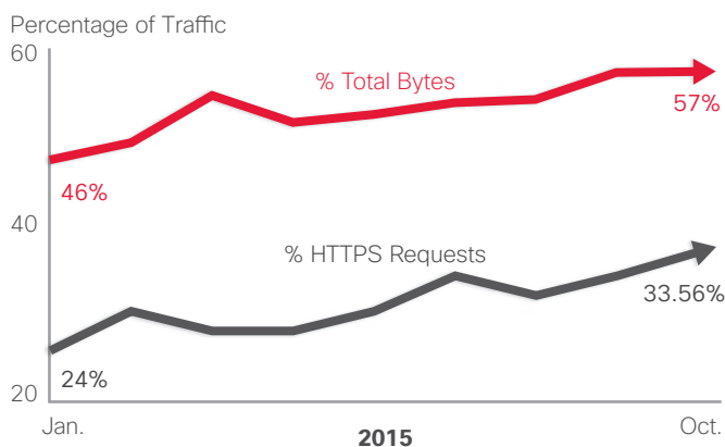
Figure 25. SSL Percentages
