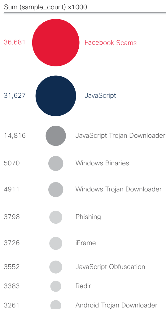
Figure 16. Most Commonly Observed Malware
