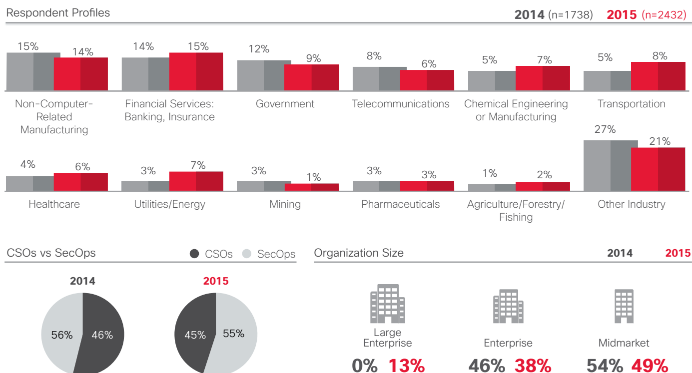
Figure 71. Respondent Profiles
