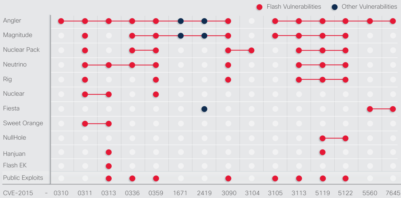
Figure 20. Common Vulnerabilities
