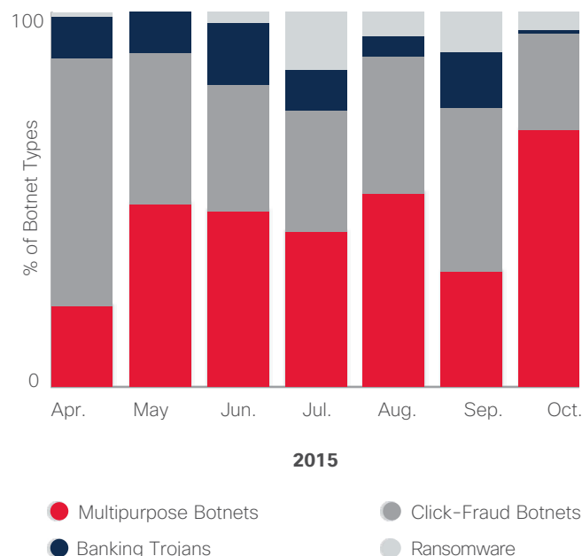
Figure 12. Monthly Threat Coverage, Based on Threat Categories
