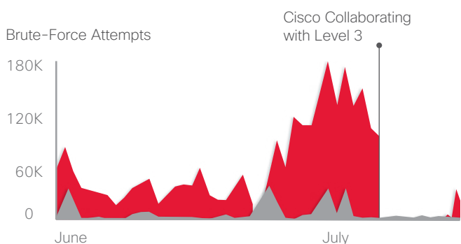
Figure 8. SSHPsychos Traffic Drops Dramatically After Intervention
