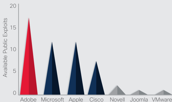
Figure 19. Number of Public Exploits Available by Vendor Vulnerability
