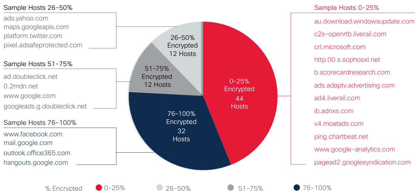
Figure 27. Top Hosts Encrypting HTTPS Traffic
