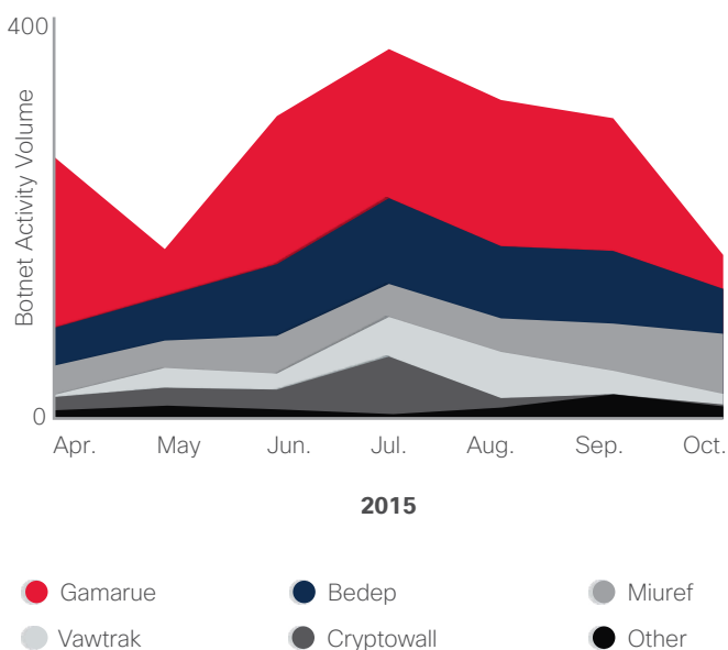
Figure 10. Growth of Individual Threats (Ratio of Infected Users)
